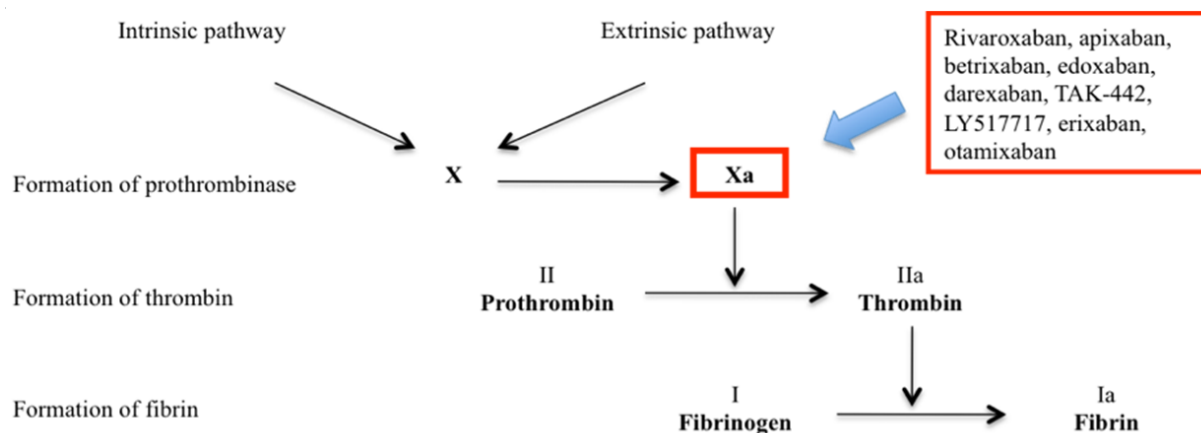
Figure 1. Schematic representation of the coagulation cascade and site of action of the novel anticoagulants.
