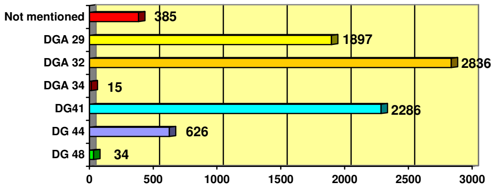
Figure 1. Teacher-librarians grades.
